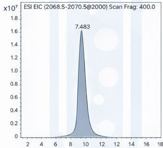
Fig.2. EIC Chromatography of Retatrutide
