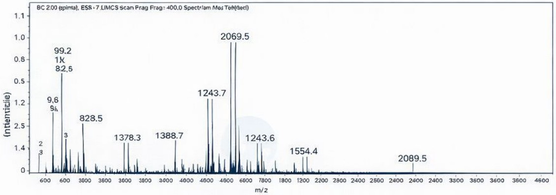
Fig.1. MS spectrum of Retatrutide
